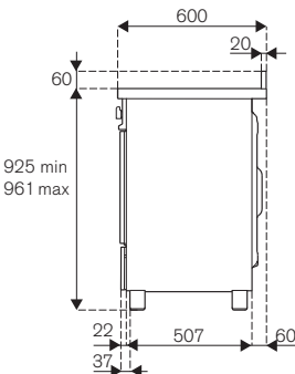
PRO64L1EART
