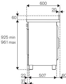
PRO96L1EART
